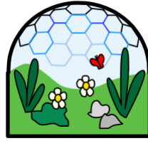
biomes
