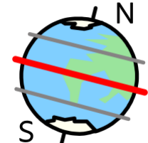
equator
